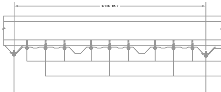
R PANEL WALL FASTENING SCHEDULE AT BASE, INTERMEDIATE GIRTS/HAT, EAVE GIRTS/HAT AND END LAPS
