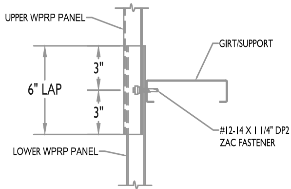
WALL PANEL END LAP DETAIL
