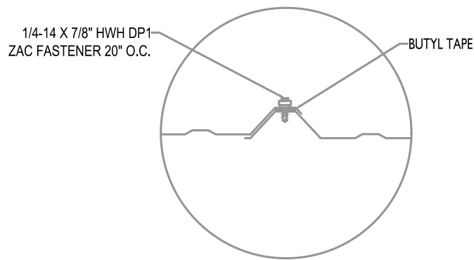
WALL PANEL SIDE LAP DETAIL
