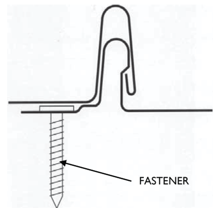
SEAM CROSS SECTION
