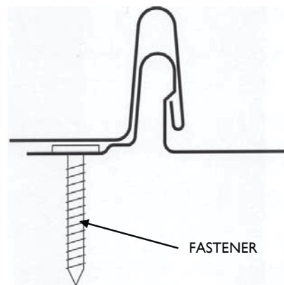
SEAM CROSS SECTION
