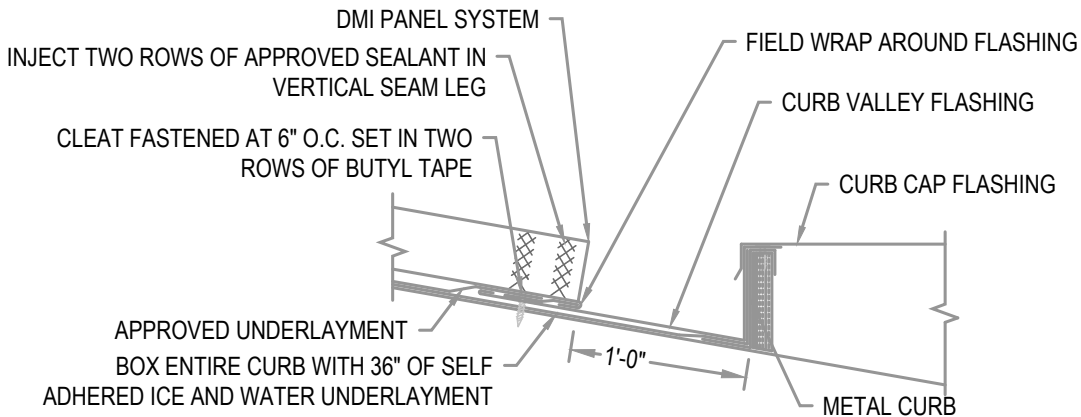
SECTION "A"
