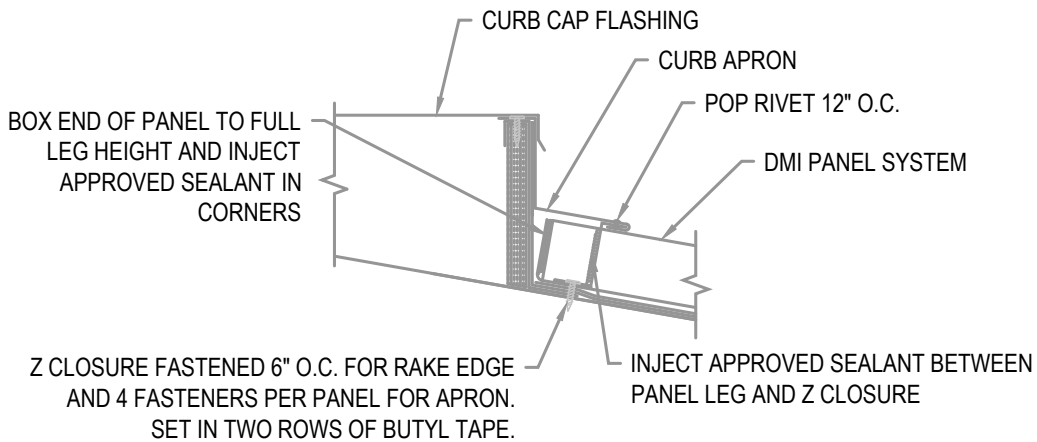
SECTION "B"
